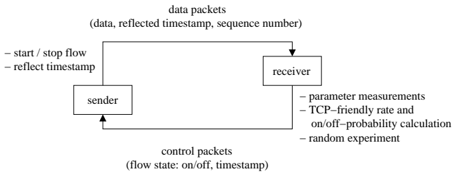
Figure 1: PCC architecture
