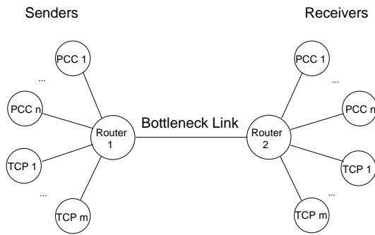
Figure 4: Simulation Topology
