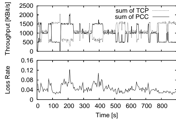
Figure 10: Throughput and Loss Rate
