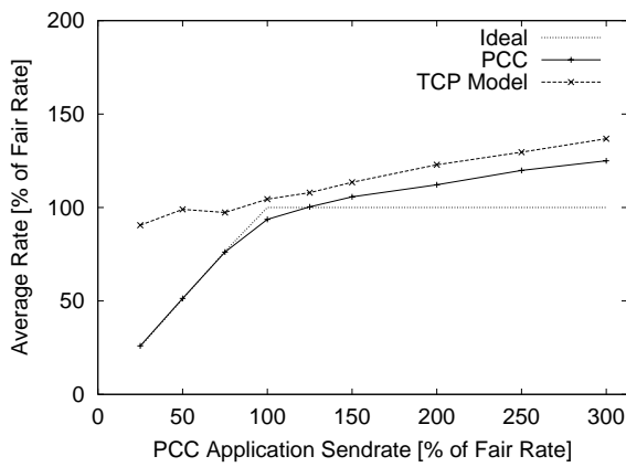
Figure 9: Comparison with Estimated TCP-Friendly Rate
