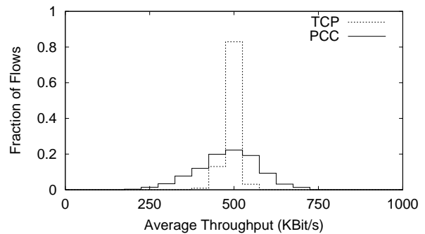
Figure 6: Distribution of Flow Throughput
